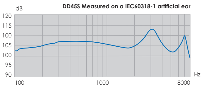
Graph 1 : Artificial Ear
