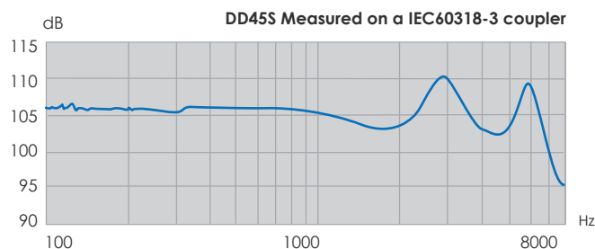
Graph 2 : Coupler
